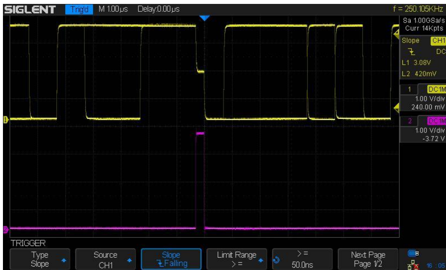
Figure 25 RUNT – Negative Edge Slope
